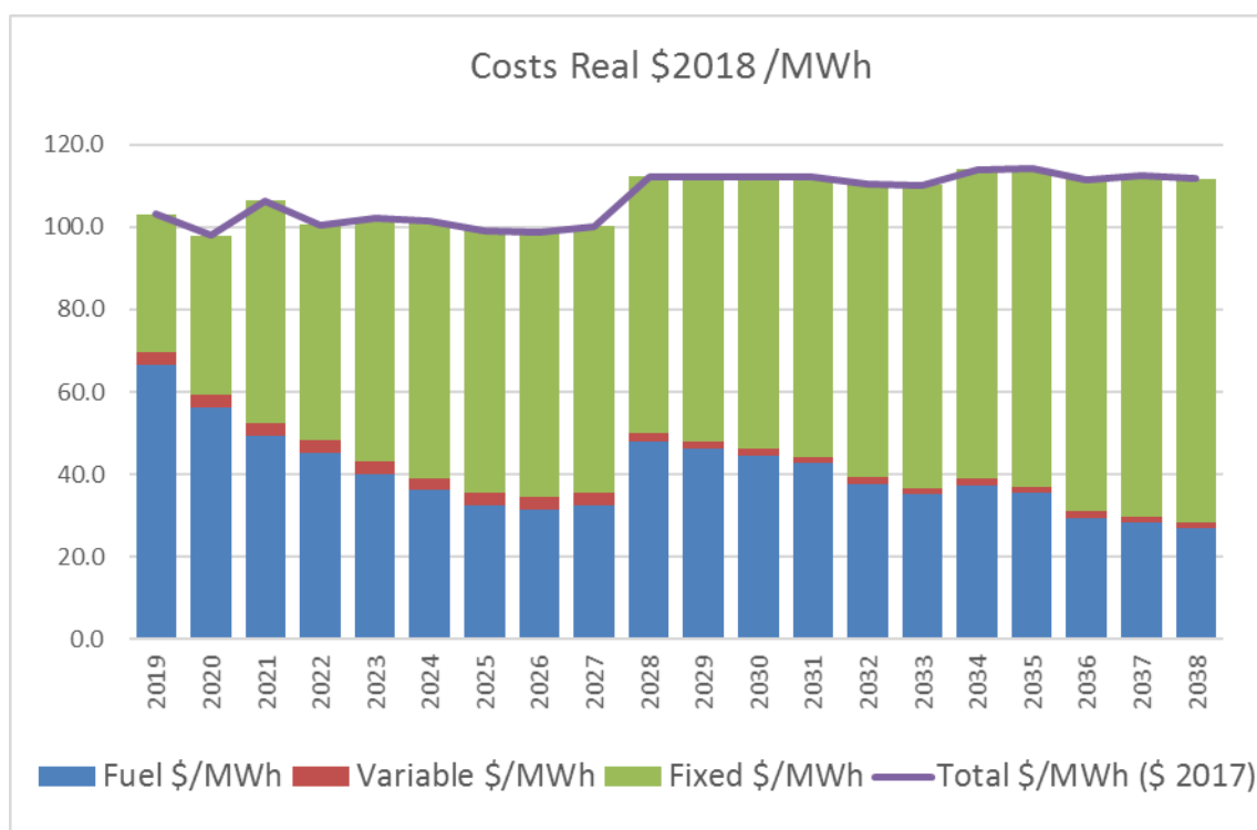
Exhibit 8-70: Scenario 1 Production Costs
