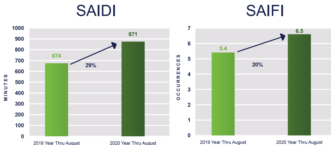
Figure 5. 2020 to 2019 SAIDI Comparison (left) and 2020 to 2019 SAIFI Comparison (right) based on LUMA calculations using industry standards
