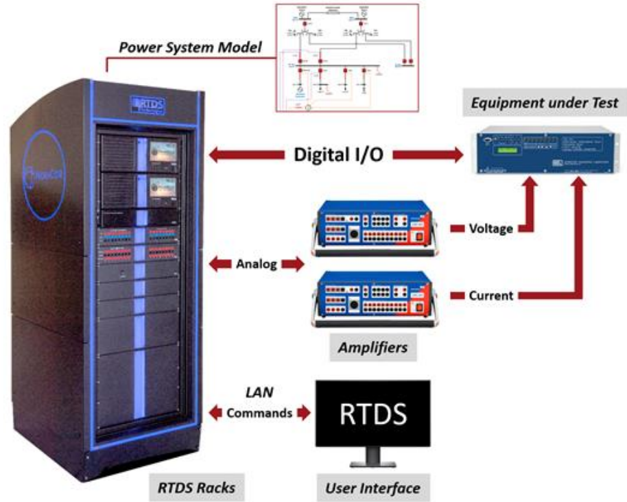
Figure 2 - Test Bed with Real Time Simulation
