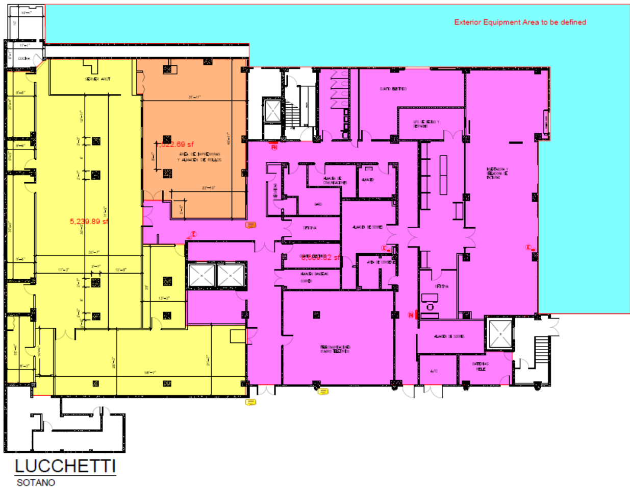
Figure 1 - Luchetti Building Basement - Areas Assigned to Test Lab
