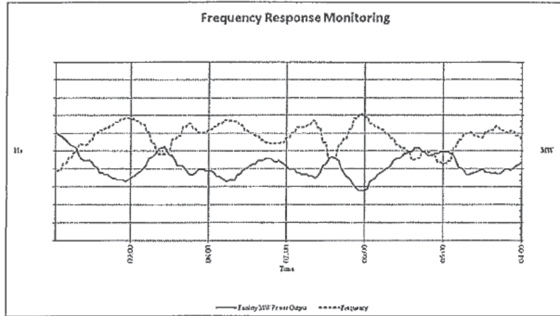
Figure 5 Frequency Response and Regulation Requirement
