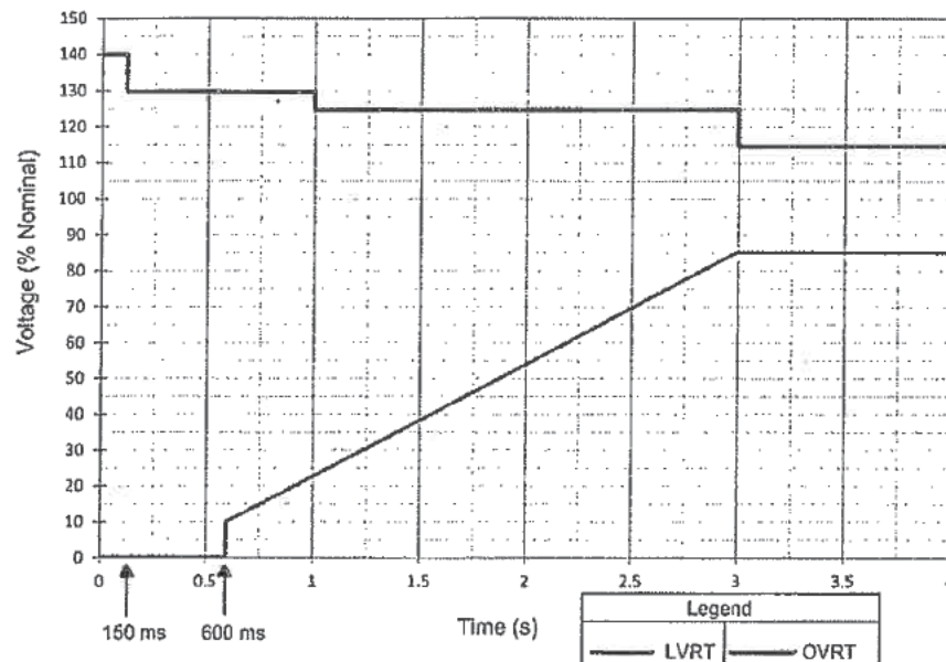
Figure 2 Voltage Ride-Through Requirements
