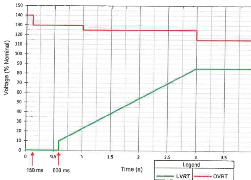
Figure 1 Voltage Ride-Through Requirements
